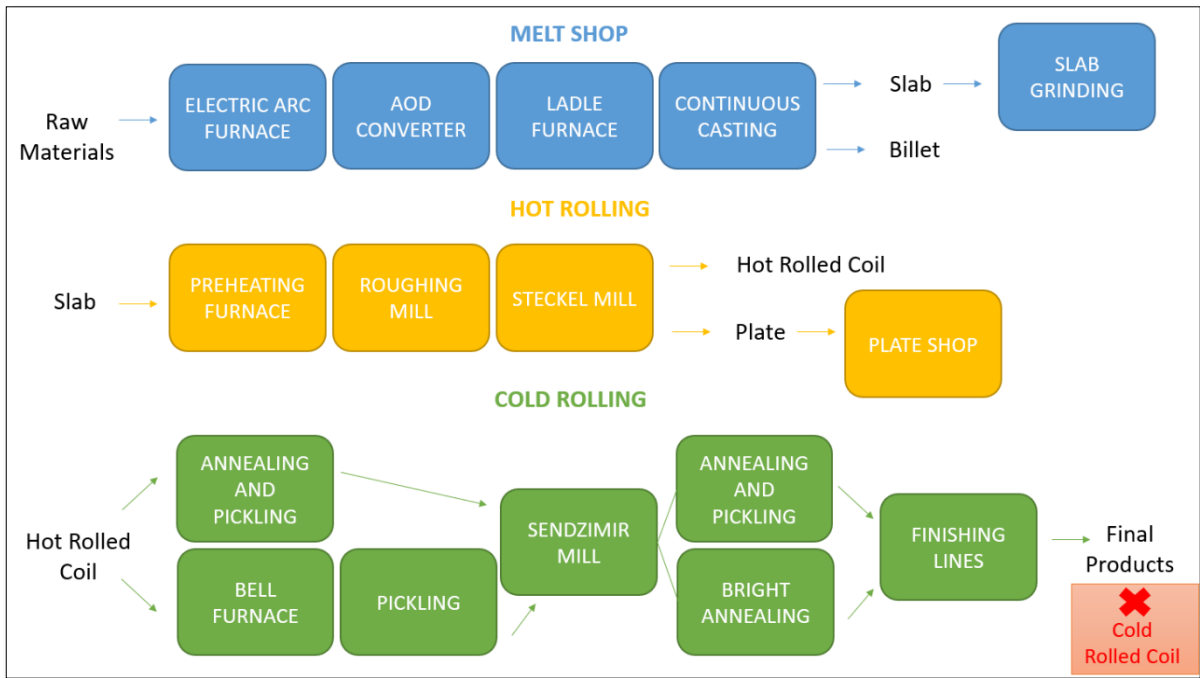
Figure 2: Cold rolling process.
